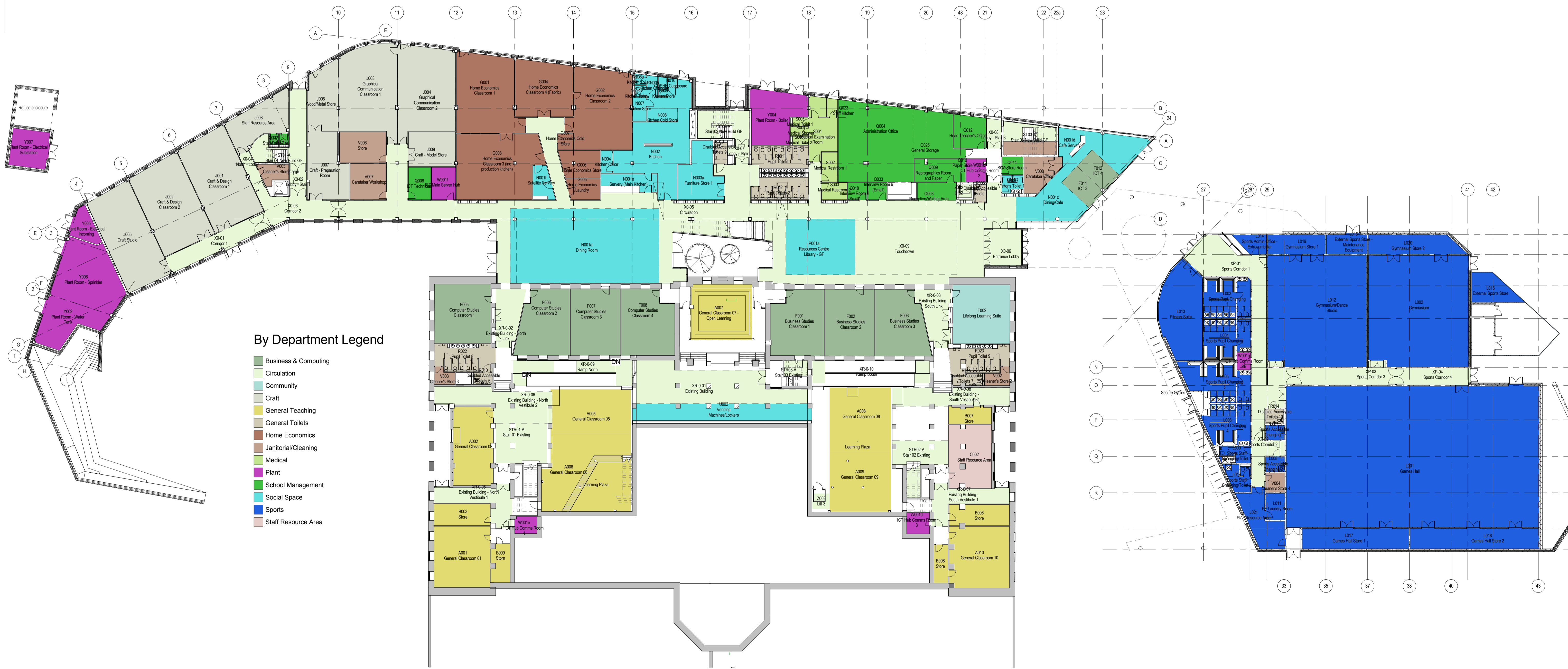
Level +00 plan
